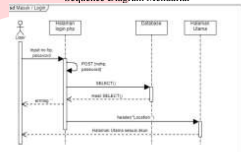
GAMBAR 10 Sequence Diagram Masuk
