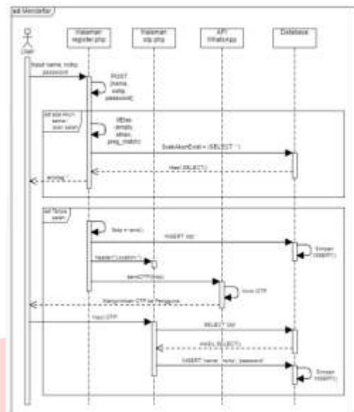
GAMBAR 9 Sequence Diagram Mendaftar
