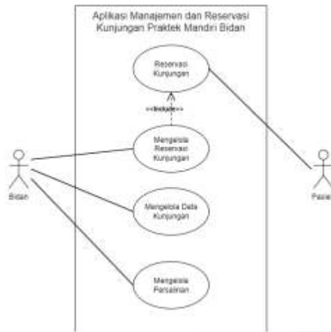
GAMBAR 8 Use Case Diagram
