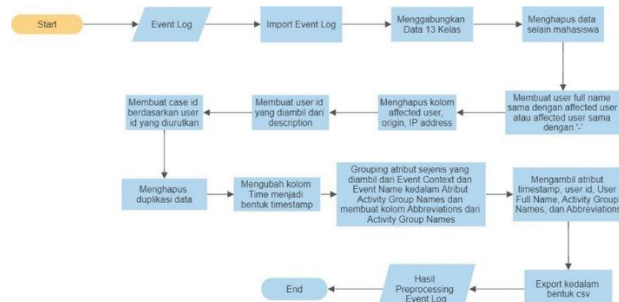
GAMBAR 5. Flowchart Preprocessing
