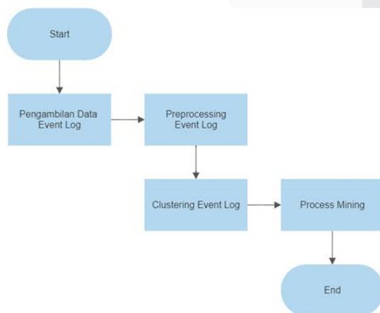
GAMBAR 4. Flowchart
