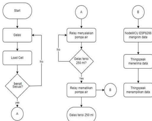
GAMBAR 3.2 Flowchart Sistem
