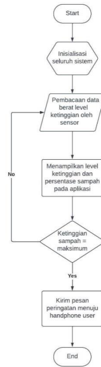
GAMBAR 3 Flowchart Monitoring Ketinggian Sampah
