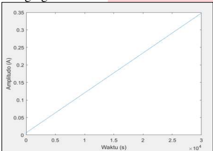
GAMBAR 3.1 Grafik step respons proses charging
