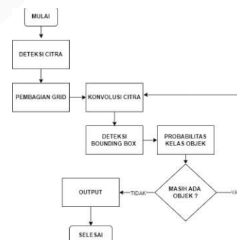
GAMBAR III.2 Flowchart Sistem
