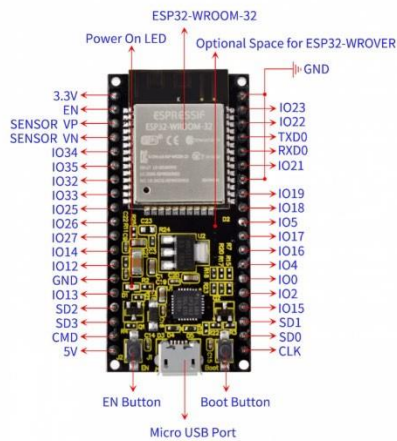
Gambar 3. ESP32
