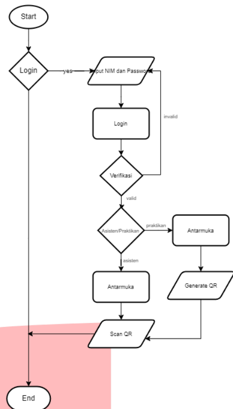
GAMBAR III. 3 Flowchart Sistem
