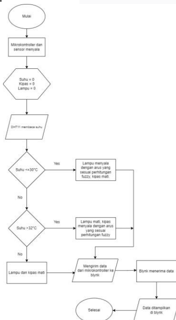
GAMBAR 10 Flowchart Sistem
