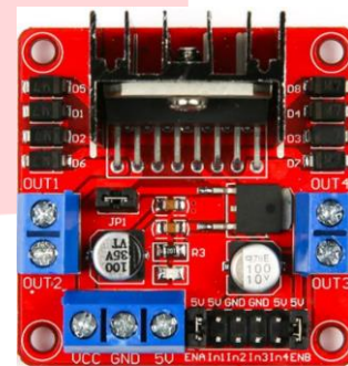
GAMBAR 8 DC Stepper Driver Controller
