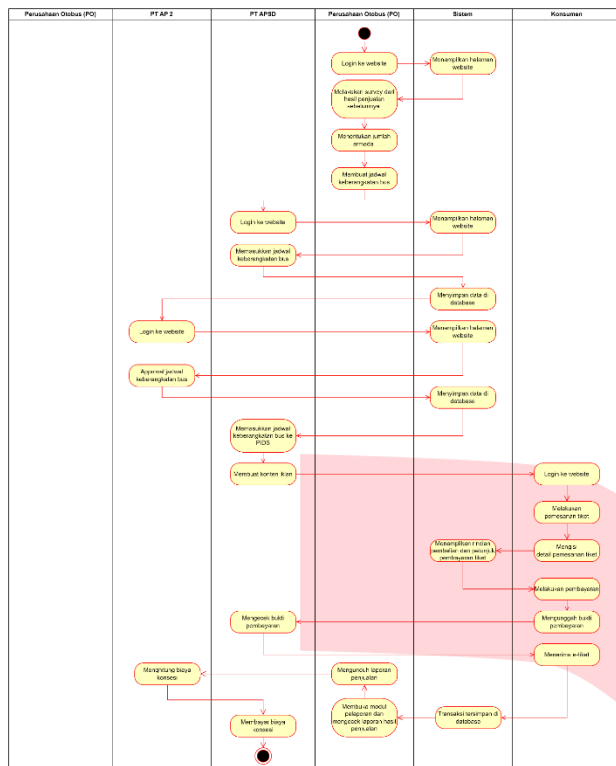
Gambar 16 Activity Diagram
