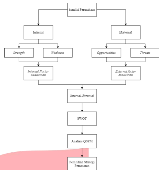
GAMBAR III.1 Model Konseptual
