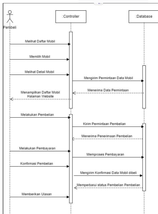
GAMBAR 7 Sequence Diagram Pembeli
