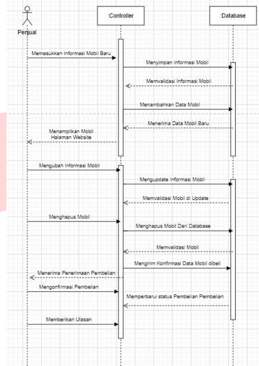
GAMBAR 8 Sequence Diagram Penjual
