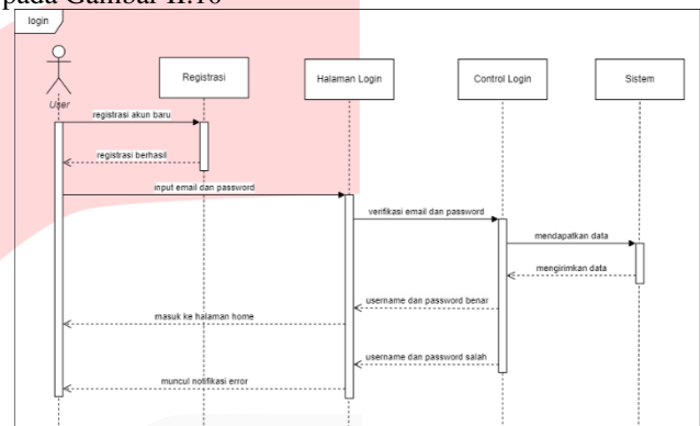
GAMBAR II.10. Sequence diagram
