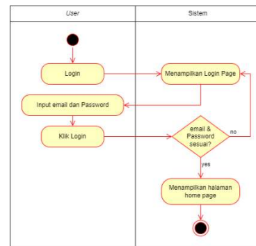
GAMBAR II.9. Activity diagram
