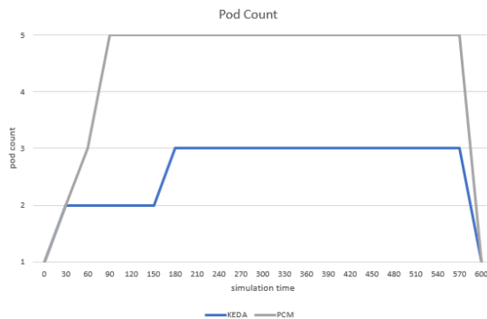
GAMBAR 8 POD COUNT
