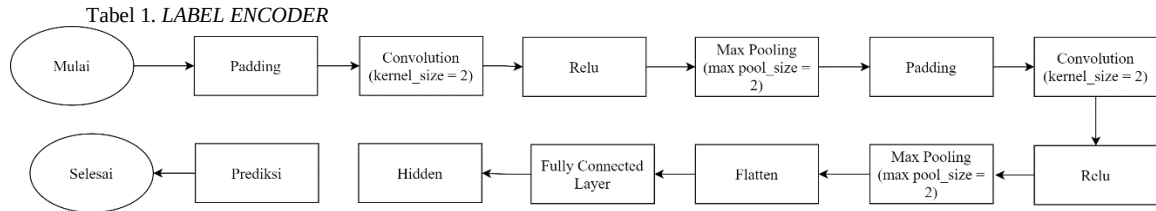
GAMBAR 8. FLOWCHART 1D-CNN
