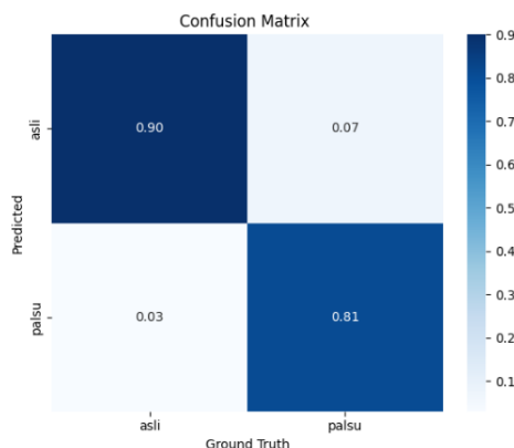
GAMBAR 5 CONFUSION MATRIX
