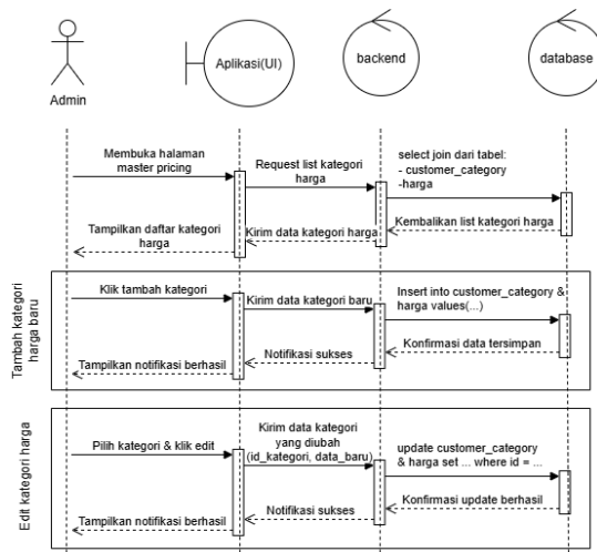
GAMBAR 8. ALUR KERJA HALAMAN MASTER PRICING
