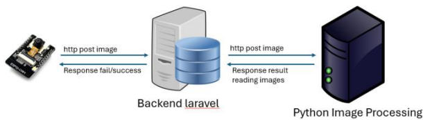
GAMBAR 4. RANCANGAN SOFTWARE
