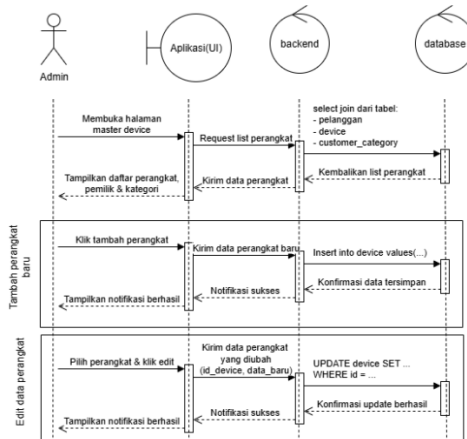
GAMBAR 9. ALUR KERJA HALAMAN MASTER DEVICE
