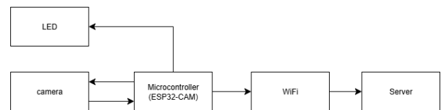
GAMBAR 2. BLOK DIAGRAM
