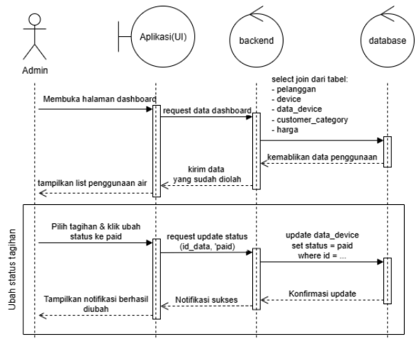
GAMBAR 6 ALUR KERJA HALAMAN DASHBOARD ADMIN
