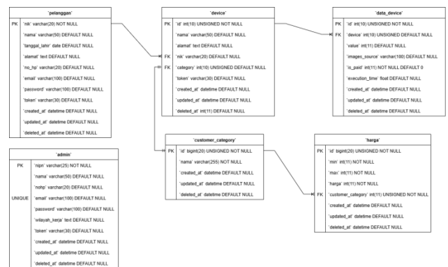
GAMBAR 10. ERD DATABASE
