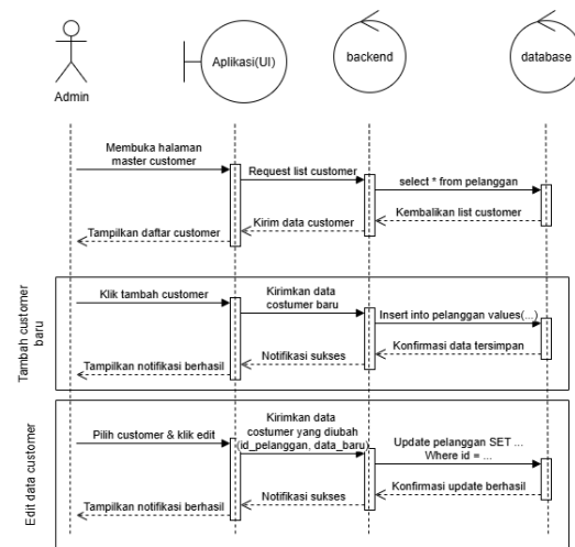
GAMBAR 7. ALUR KERJA HALAMAN MASTER CUSTOMER
