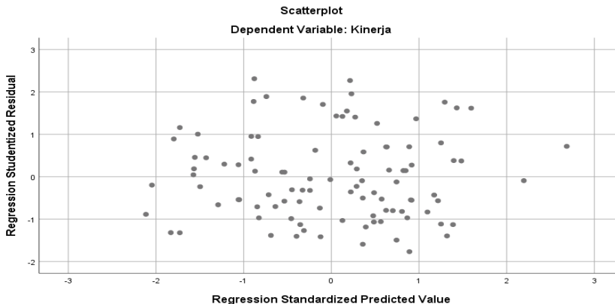
Gambar 2. Uji Scatterplot
