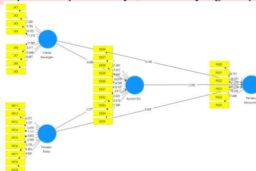
Gambar 4.1 Hasil Uji Outer Model
