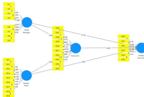
Gambar 4.2 Hasil Uji Inner Model Sumber: Hasil Olahan Peneliti (2025)
