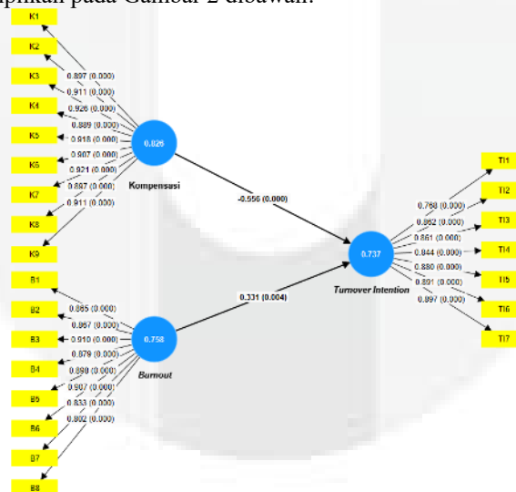
Gambar 2. Graphical Output Model SEM-PLS
