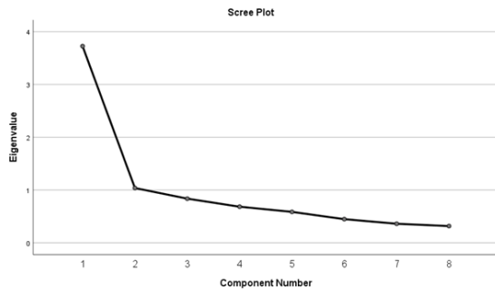
Gambar 2 Scree Plot
