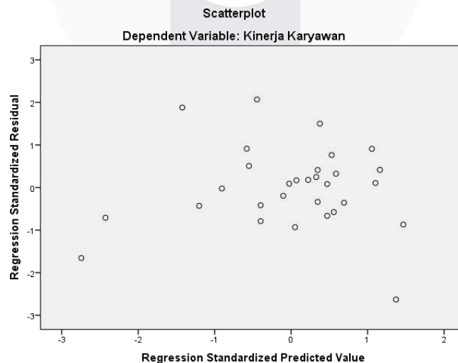
Gambar 4.3 Diagram Pencar
