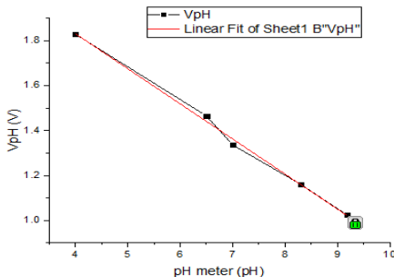
GAMBAR 7 KALIBRASI SENSOR pH
