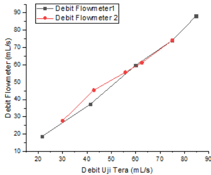
GAMBAR 6 KALIBRASI SENSOR FLOWMETER
