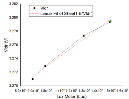
GAMBAR 9 KALIBRASI SENSOR LDR
