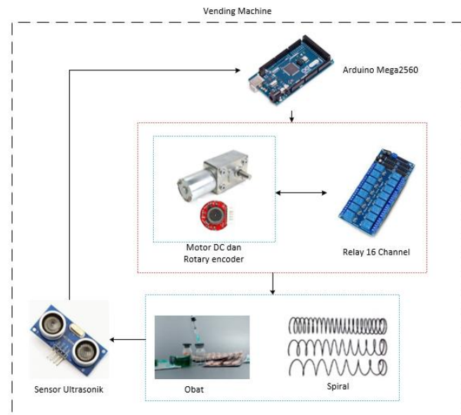
GAMBAR 1 BLOK DIAGRAM
